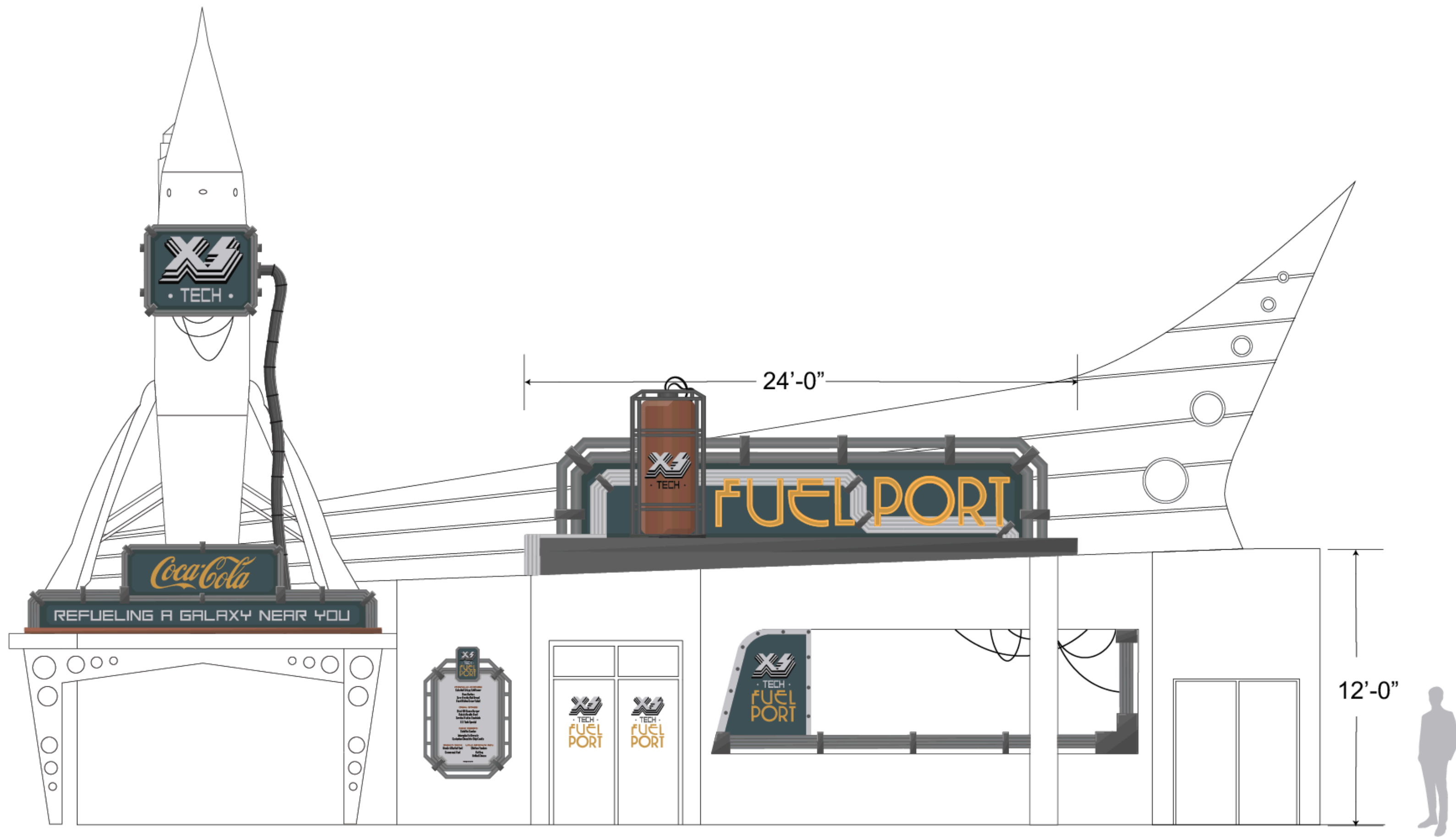
FRONT ELEVATION
